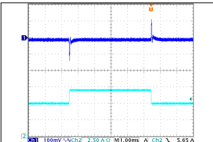
Figure 5: Output voltage response to step-change in load current (50%-75%-50% of I out (max); dI/dt = 0.1 A/μs). Load cap: 1 μF ceramic and 15 μF tantalum capacitors. Ch 1: V out , Ch 2: I out (2.5A/div).
