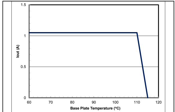
Figure 4: maximum load current vs. baseplate temperature when conductively cooled. Note: The system design must provide a suitable thermal path that maintains the baseplate temperature below 100°C.
