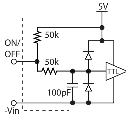
Figure B: Internal ON/OFF pin circuitry
