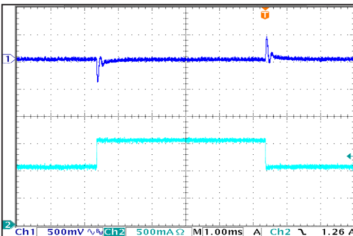
Figure 5: Output voltage response to step-change in load current (50%-75%-50% of I out (max); dI/dt = 0.1 A/μs). Load cap: 1 μF ceramic capacitor. Ch 1: V out , Ch 2: I out (0.5A/div).
