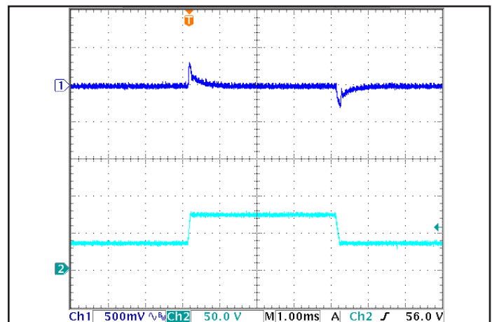
Figure 6: Output voltage response to step-change in input voltage (1V/ \mu s ). Load cap: 1 \mu F ceramic and 15 \mu F tantalum capacitors. Ch 1: V_{out} , Ch 2: V_{in} .
