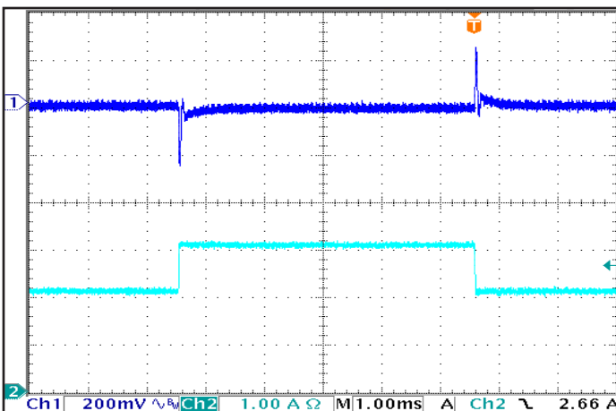
Figure 5: Output voltage response to step-change in load current (50%-75%-50% of I_{out(max)} ; dI/dt = 0.1 A/\mu s ). Load cap: 1 \mu F ceramic and 15 \mu F tantalum capacitors. Ch 1: V_{out} , Ch 2: I_{out}(1.0A/div) .
