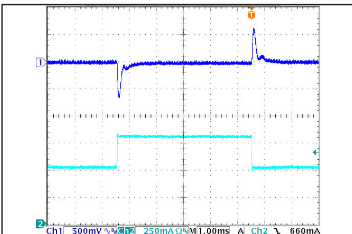
Figure 5: Output voltage response to step-change in load current (50%-75%-50% of Iout(max); dI/dt = 0.1 A/μs). Load cap: 1 μF ceramic capacitor. Ch 1: Vout, Ch 2: Iout(0.25A/div).
